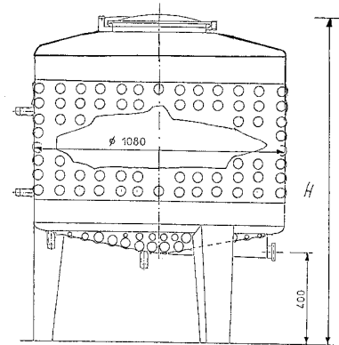
Version 2 manhole Ø 400 mm
